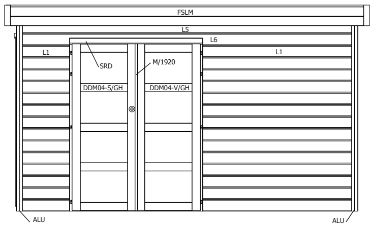
FACADE
